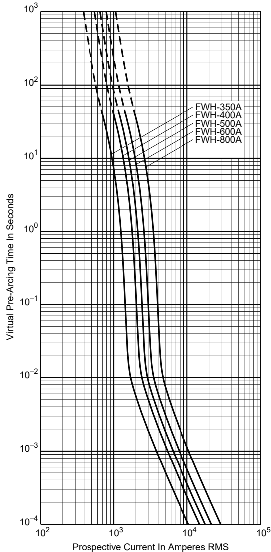
Time-current curve - 350 A to 800 A
