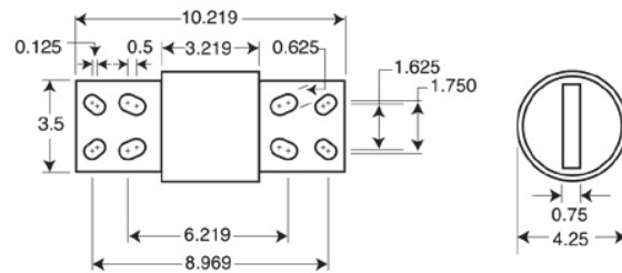
Dimensions (in) - 1400 A and 1600 A
